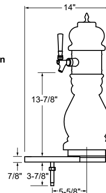
Side Elevation
