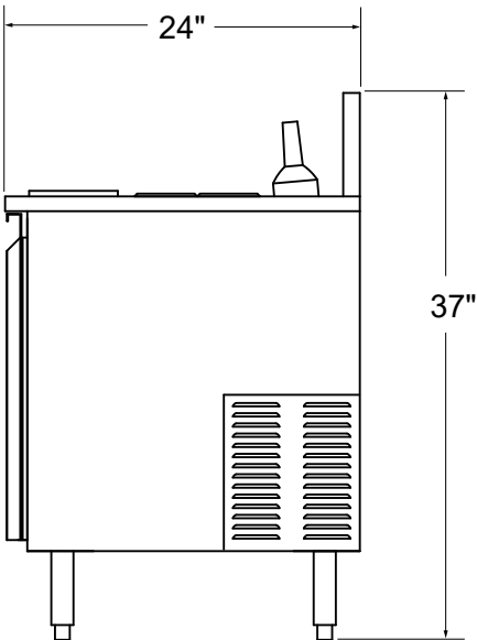
Side Elevation
