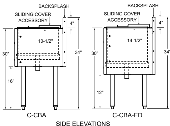
SIDE ELEVATIONS
