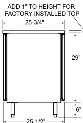
Side Elevation
