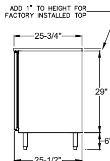
Side Elevation
