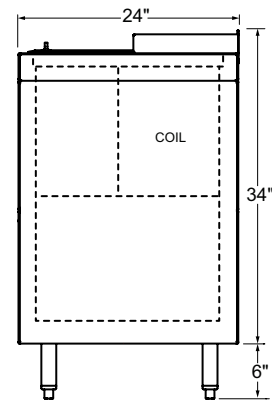
MF36, MF48 Side Elevation
