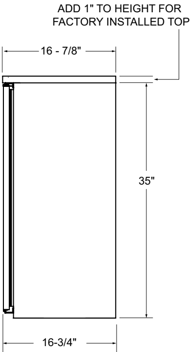
Side Elevation
