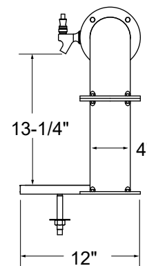
Side Elevation
