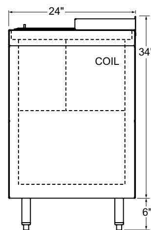
ST36, ST48, ST60, ST72, ST96 Side Elevation
