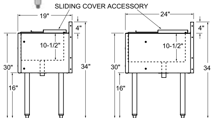
C-IBA SIDE ELEVATIONS C-IBB
