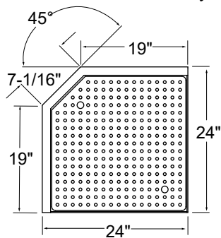
CIR-24/24 with chamfered back corner
