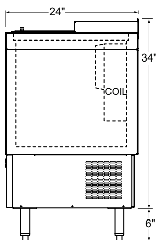
ST24 Side Elevation
